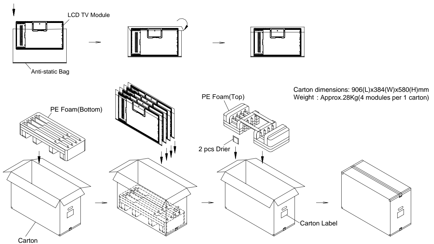
Figure.9-1 packing method
